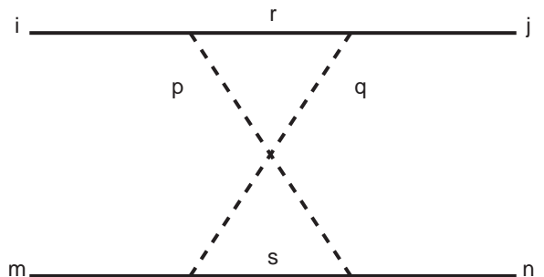
FIG. 7: Octet representation indices TME-crossed-graphs. The solid lines denote quarks with labels i, m, j, n, r, s . The dashed lines with labels p, q refers to the pseudo-scalar mesons.
