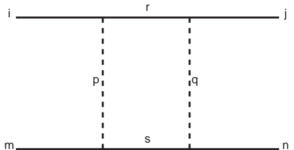
FIG. 6: Octet representation indices TME-parallel-graphs. The solid lines denote quarks with labels i, m, j, n, r, s . The dashed lines with labels p, q refers to the pseudo-scalar mesons.
